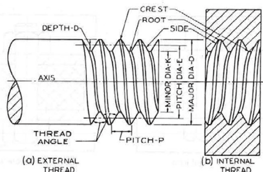
Figure 1- Thread Nomenclature
