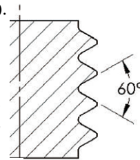
Figure 2- Unified Series Thread Profile
