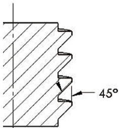
Buttress Thread
