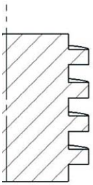
Square Thread
