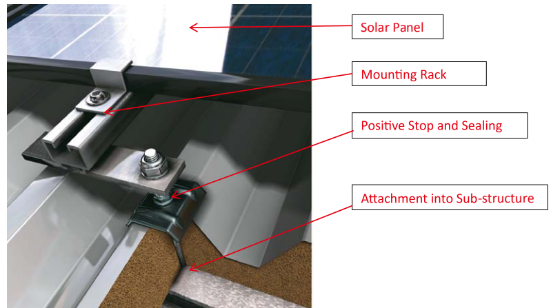
Figure 2 (EJOT® JA3/JZ3 Solar Fastening System Installed)
