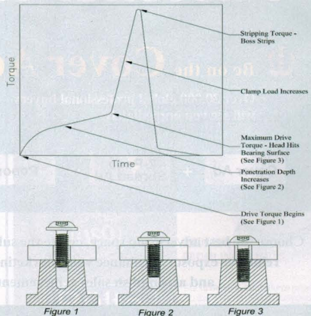
Figure 2. Explanation of Torque versus Time Plot
