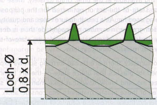
Figure 5. Relief in the Thread's Root for Displaced Material (Green Shading Represents Displaced Material)
