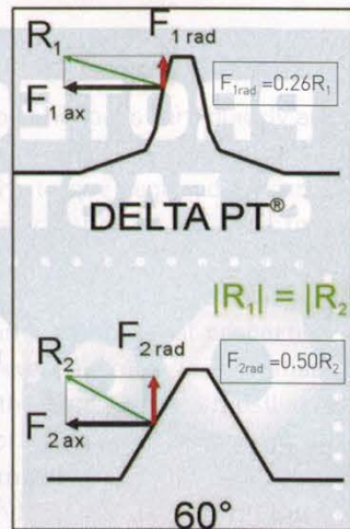
Figure 3. Comparison of Force Components on Standard 60° Thread and State-of-the-Art Thread profiles
